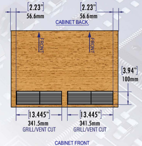
Top View Fig 6.4 (Optional Ventilation)
